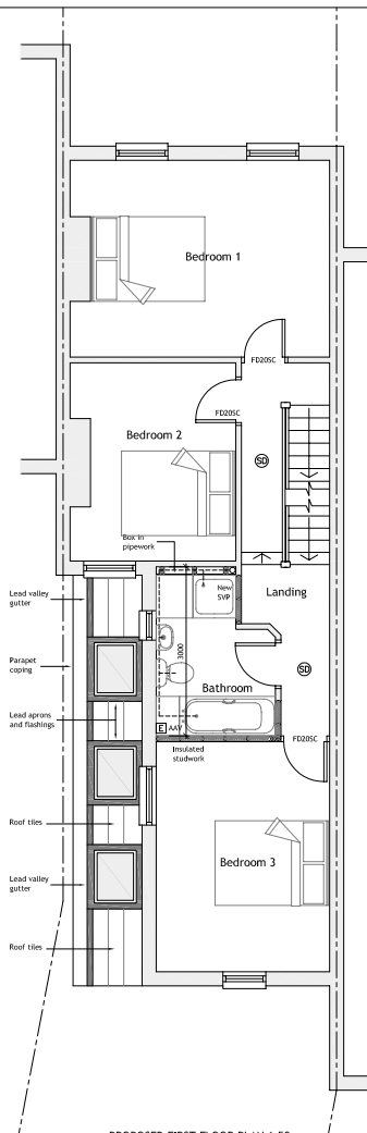
PROPOSED FIRST FLOOR PLAN 1-50
